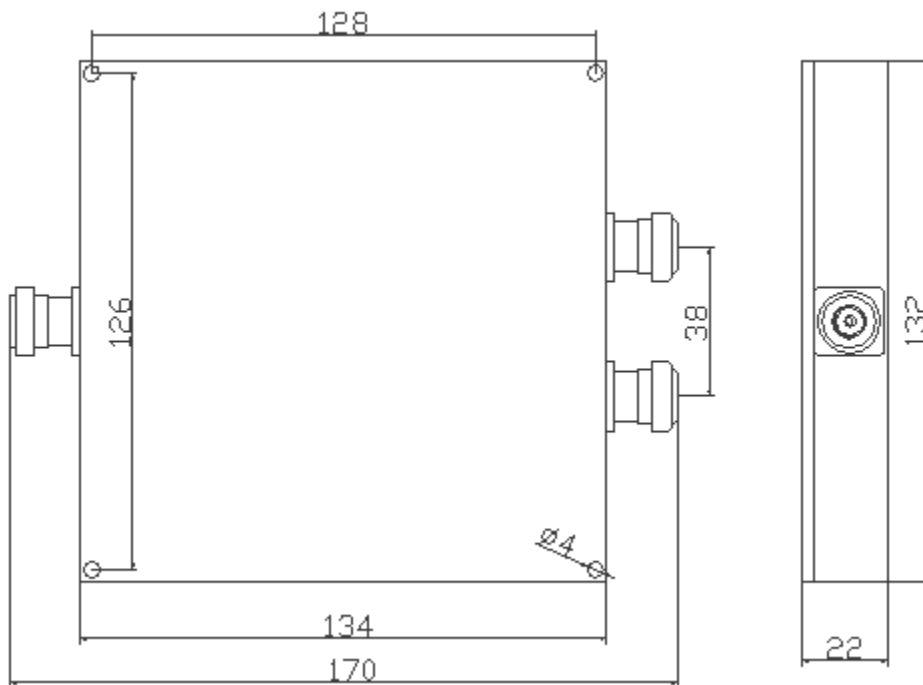
Product Drawing
